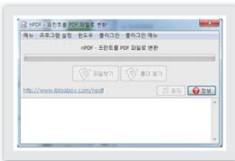
[ nPDF ]
